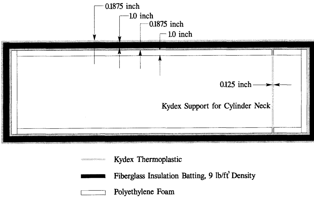
FIGURE 11. MODIFIED VIKING OVERPACK USING FIBERGLASS BATT INSULATION
