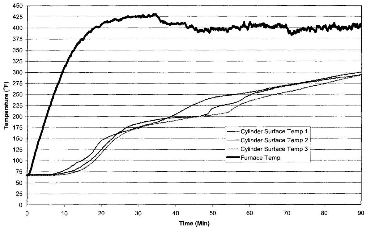
FIGURE 10. FURNACE TEST RESULTS USING 76.5-CUBIC-FOOT CYLINDER INSIDE ANVIL OVERPACK
