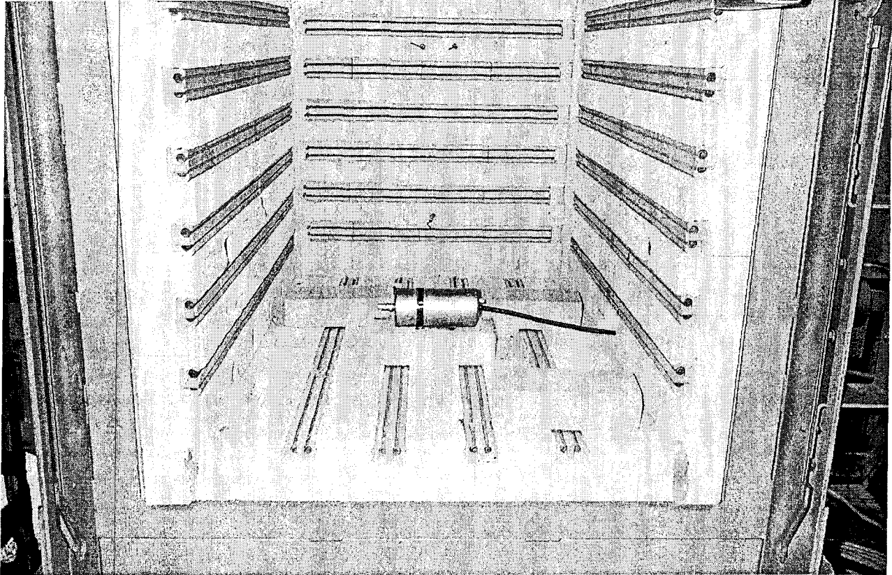
FIGURE 1. FURNACE AND OXYGEN GENERATOR
