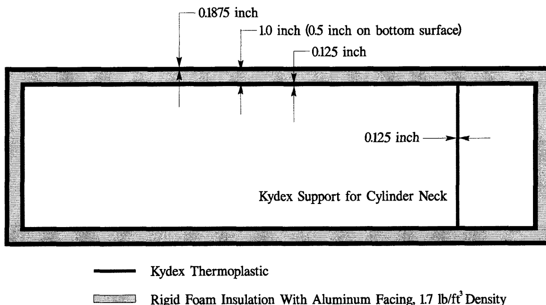
FIGURE 13. MODIFIED VIKING OVERPACK USING RIGID FOAM INSULATION
