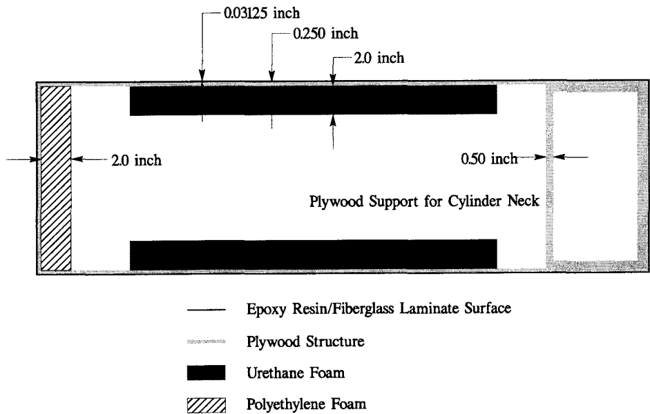
FIGURE 7. SCHEMATIC OF BILL THOMAS ASSOCIATES OVERPACK CONSTRUCTION
