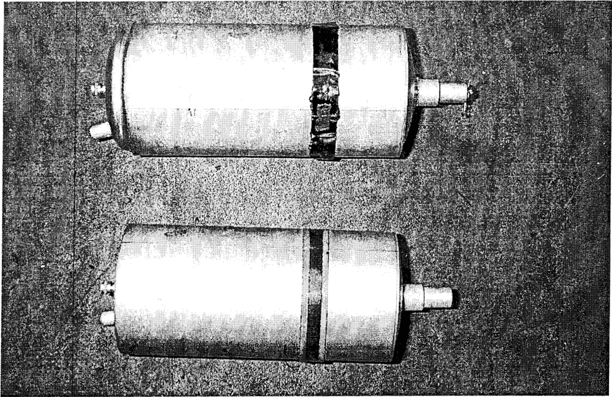
FIGURE 2. OUTWARDLY BULGED GENERATOR AND NORMAL GENERATOR
