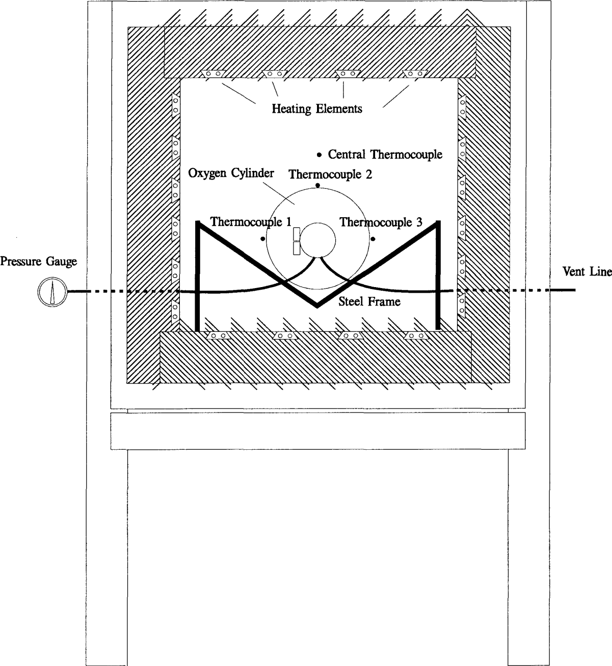
FIGURE 1. TEST FURNACE
