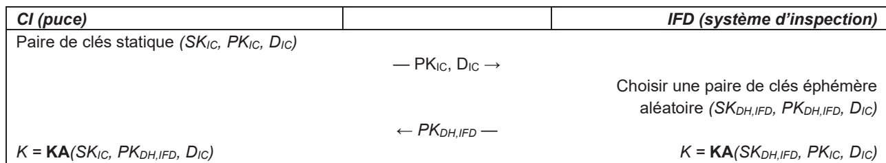
Figure 3. Authentification de la puce
