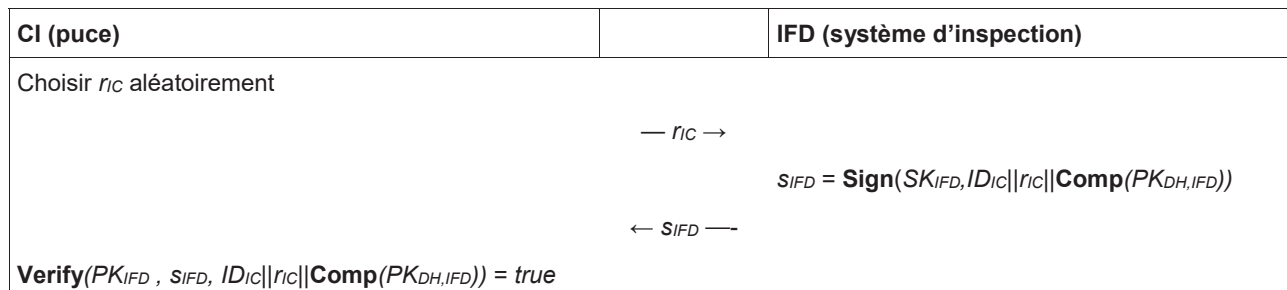
Figure 4. Authentification du terminal
