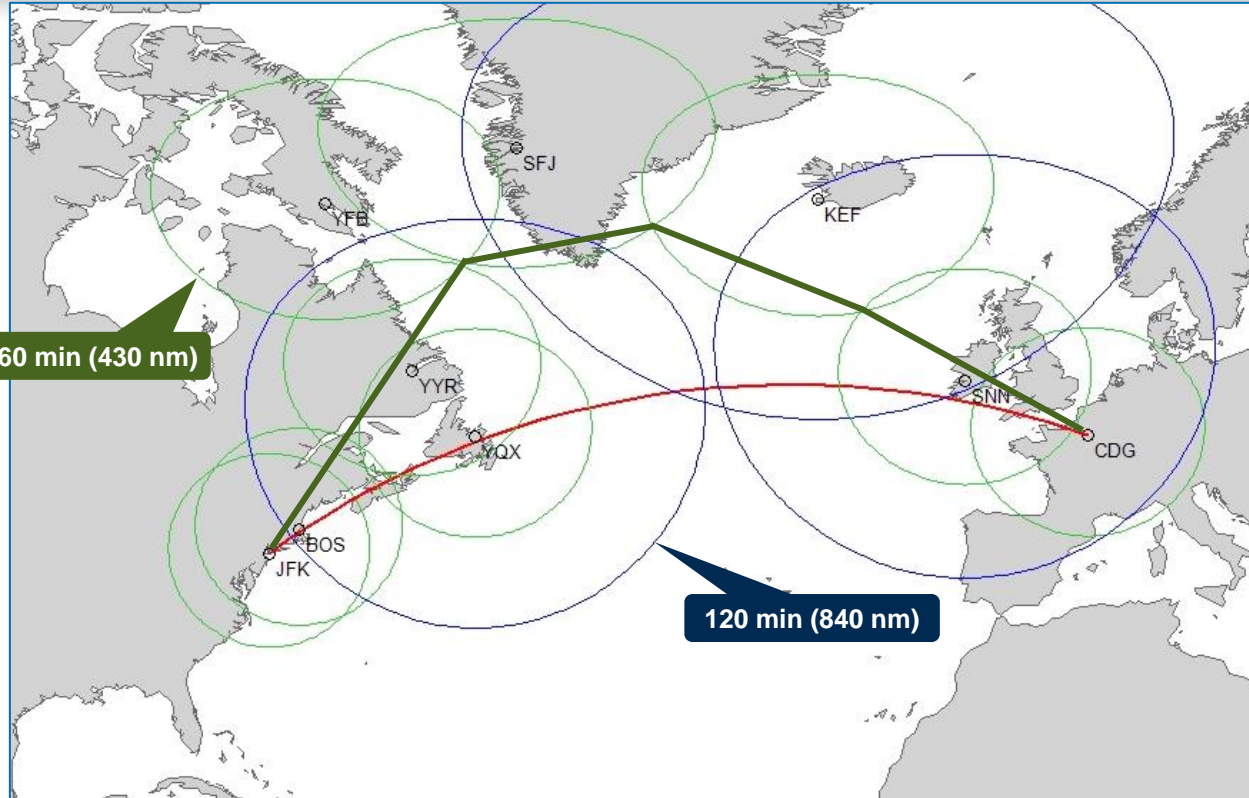
Figure 2 CDG-JFK route Non-EDTO track and EDTO 120 min track
