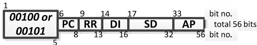
Figure 3A Uplink Format 4 and 5
