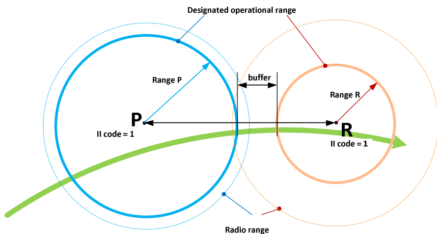
Figure 9 – Minimum separation distance between interrogators having the same II code
