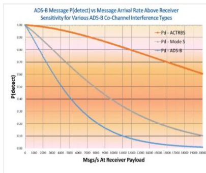
Figure 3 – ADS-B P(detect) vs Message Arrival Rate for Various Co-Channel Interference Types
