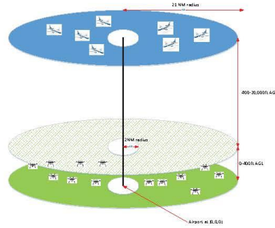
Figure 1- NAS/sUAS Airspace Simulation Approach
