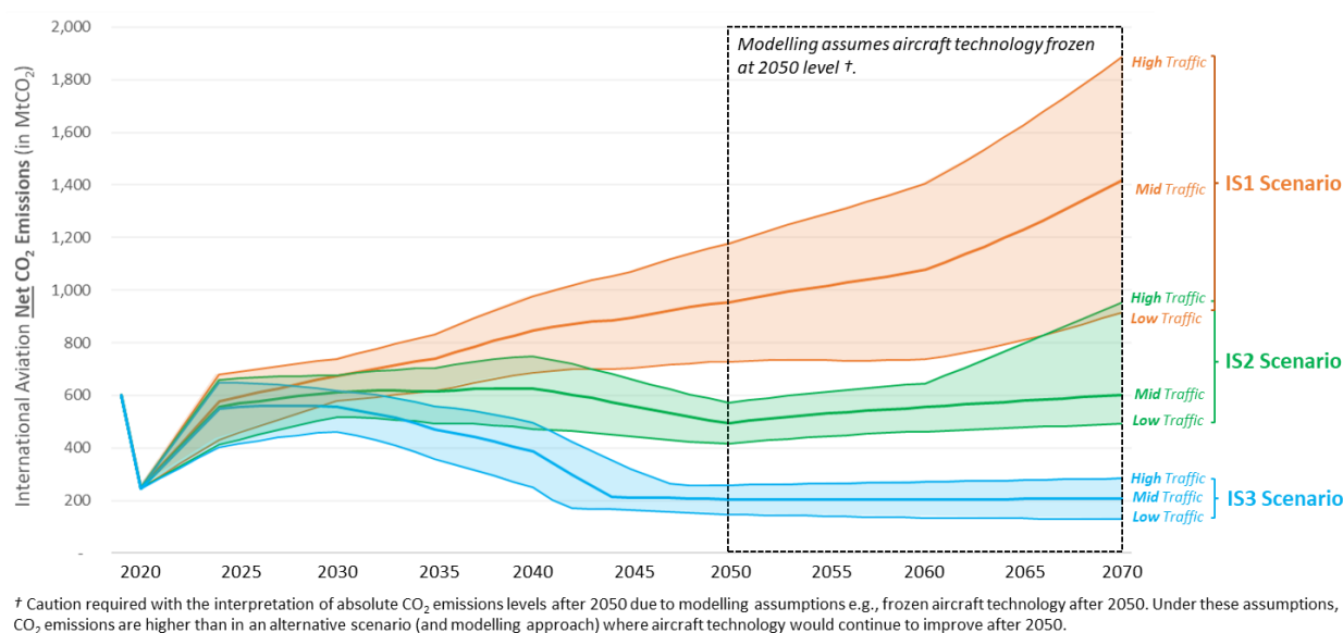
Figure 4. Effects of traffic scenarios on residual CO 2 emissions across LTAG integrated scenarios
