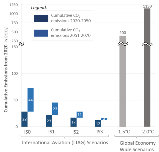
Figure 2. Cumulative CO 2 emissions from international aviation in context of 1.5°C and 2°C
