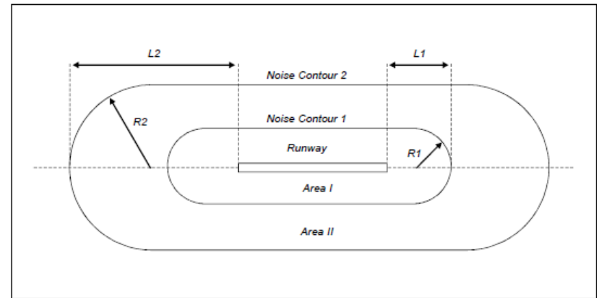
Noise contours for basic noise zoning
