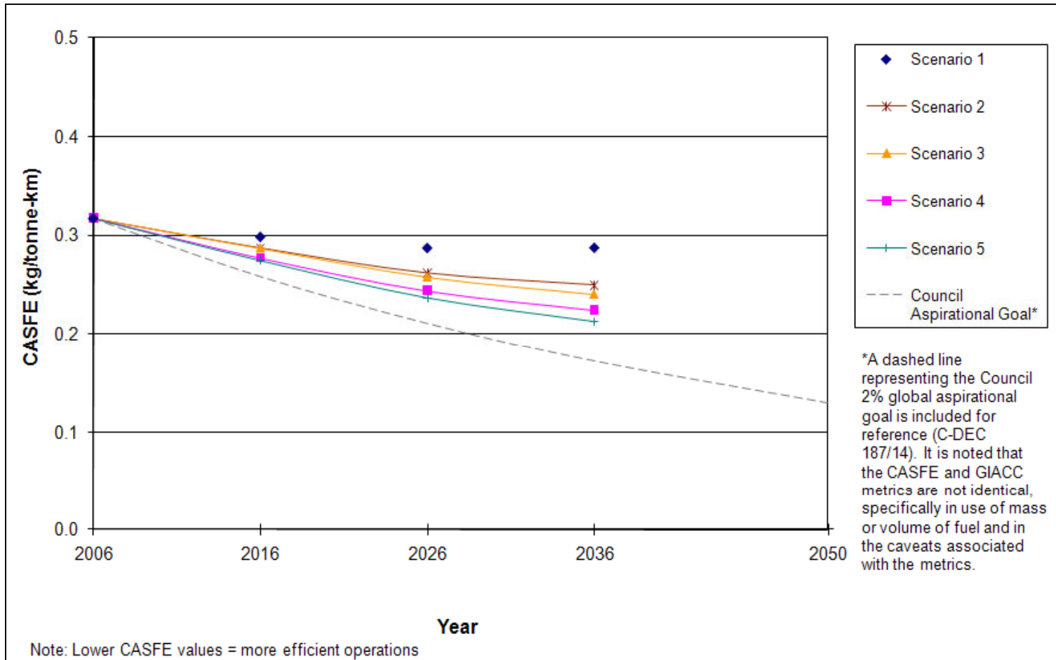
Global Commercial Aircraft System Fuel Efficiency (CASFE)
