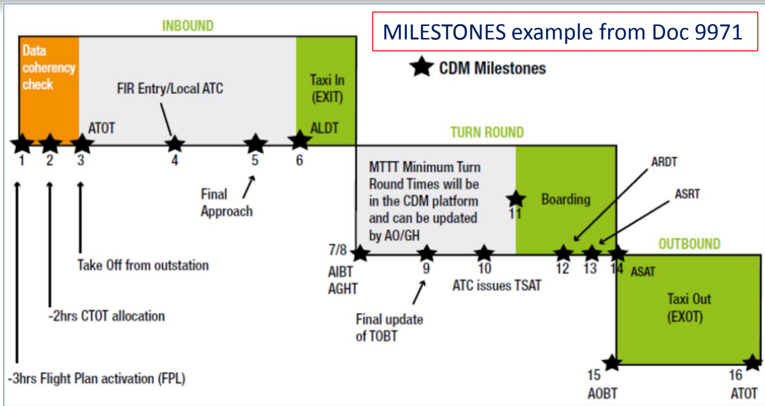
Figure III-3-2 A-CDM milestones used in Europe and other parts of the world
