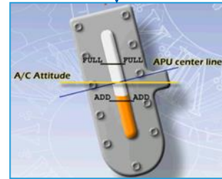
APU oil tank sight glass reading
