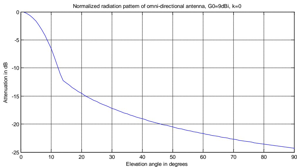
FIGURE 1 Omnidirectional base station antenna pattern in the vertical plane
