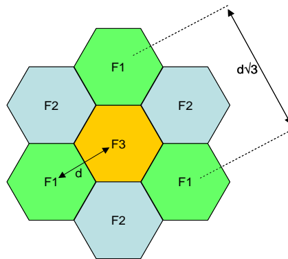
FIGURE 13 Typical frequency reuse pattern in cell structure
