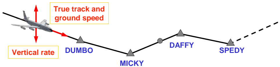
Figure 2-40. ADS-C Earth reference group
