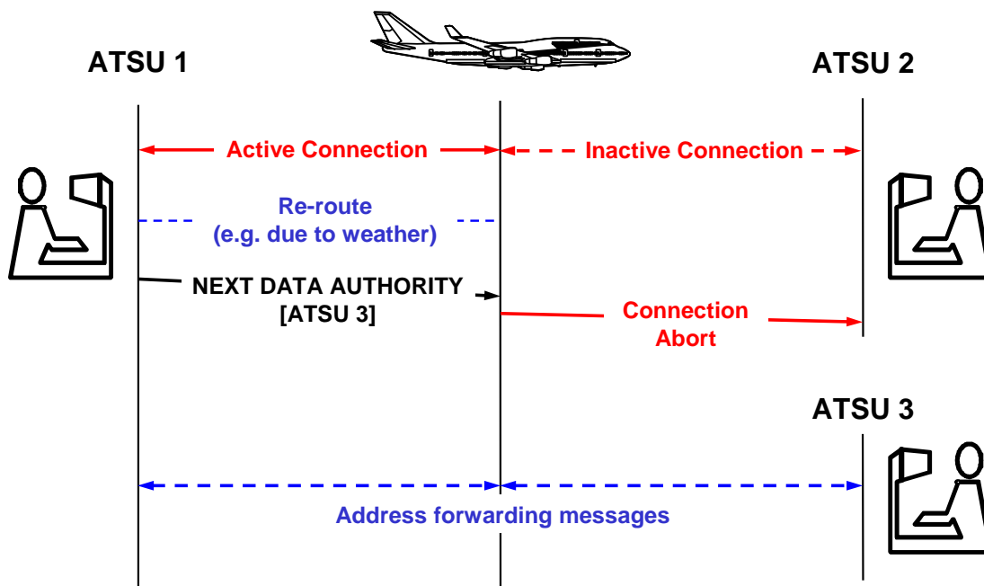
Figure 2-21. Sending a new NDA following a re-route
