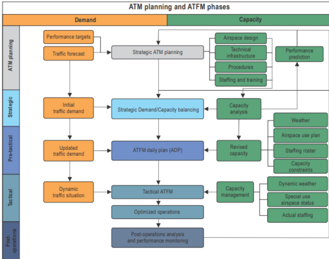
Figure II-4-1. ATM planning and ATFM phases
