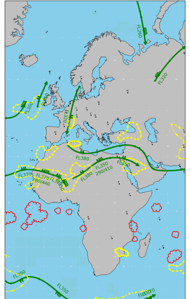
SigWx objects - WAFC: EGRR - Area: C - 2023-04-05 00Z T+06 forecast - Python objects
