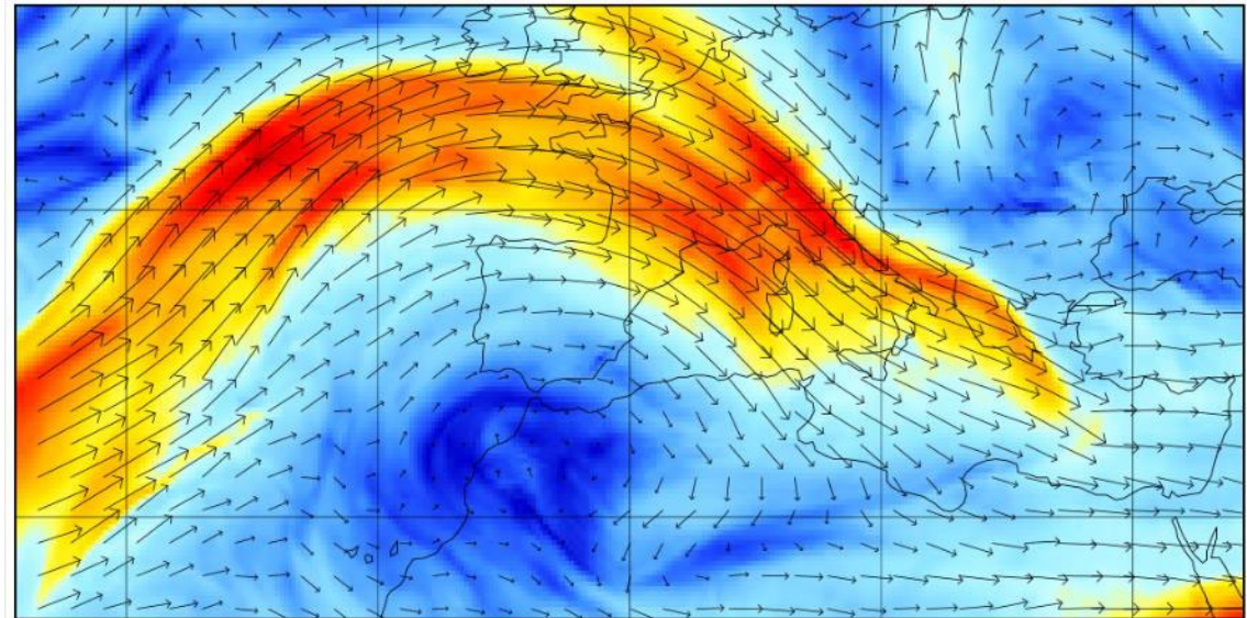
wind vector @ FL300 (300.9hPa)
