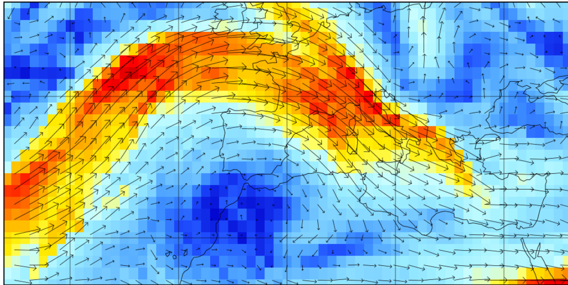
wind vector @ FL300 (300hPa)
