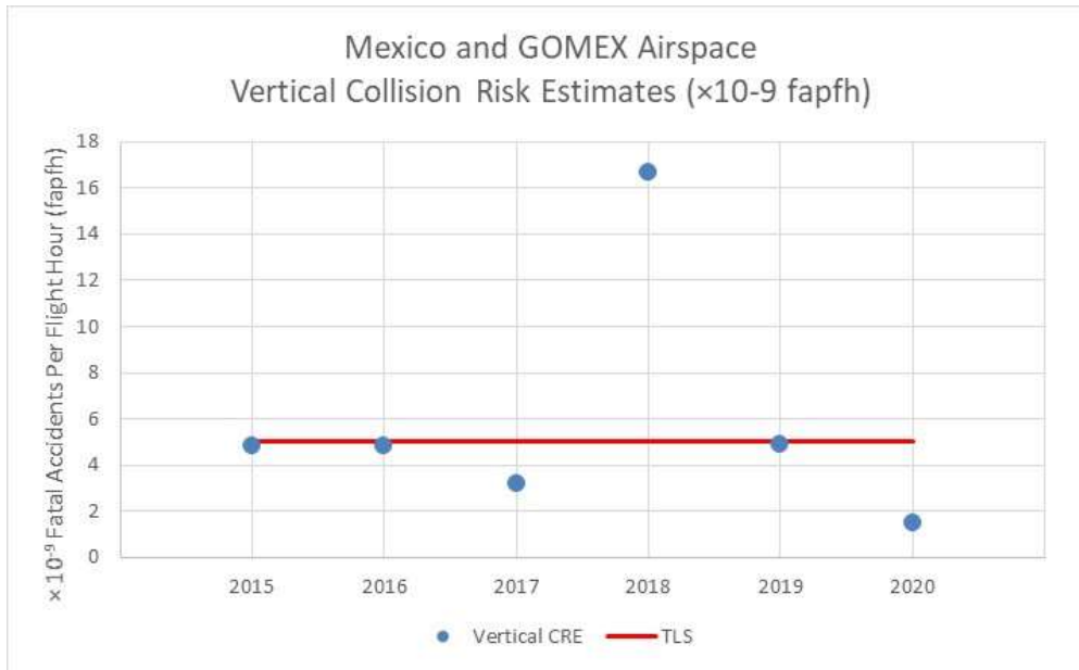
Figure 2-8. Vertical Collision Risk Estimates, Mexico and GOMEX Airspace 2015 - 2020
