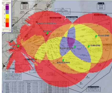
Figure 01 – Campos Basin ADS-B coverage – 500ft AMSL
