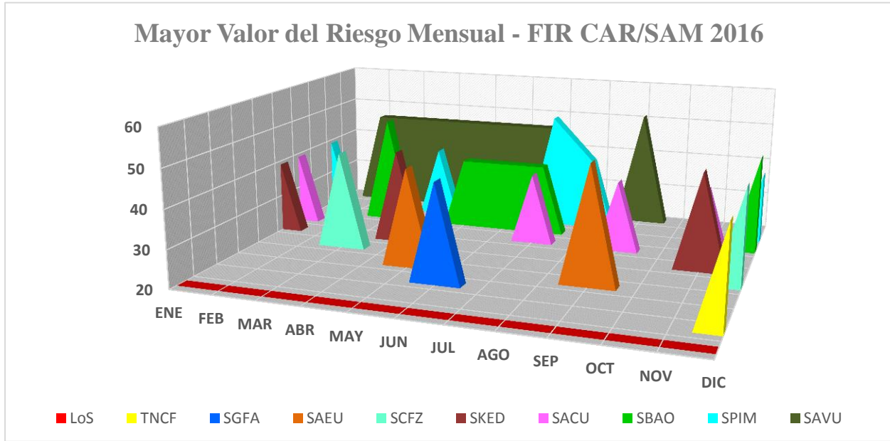
Graph 5 - Highest risk value for FIRs in CAR/SAM RVSM airspace. The red line is the VR of the LoS (20).
