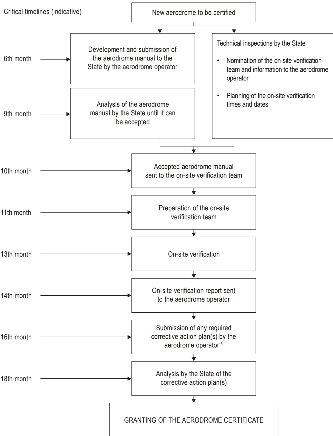
Figure 2-B-1. The certification process
