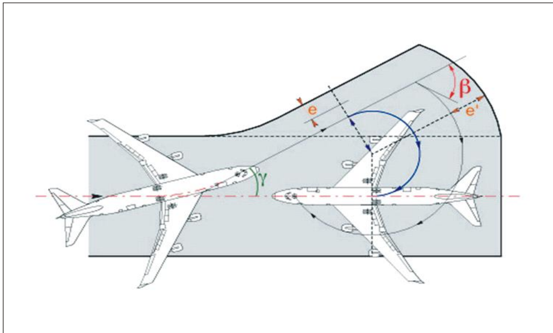
Figure 4-1. Example of minimum turn pad dimension
