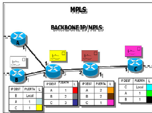
Figure 4-2: MPLS Switching
