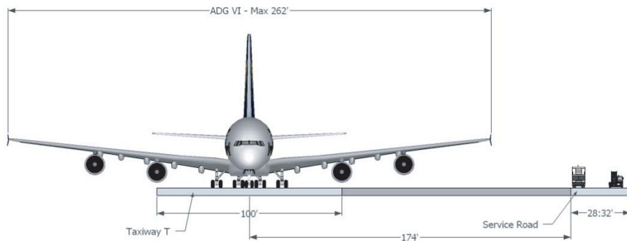
Figure H-2. Cross-section of the existing separation at ANC.
