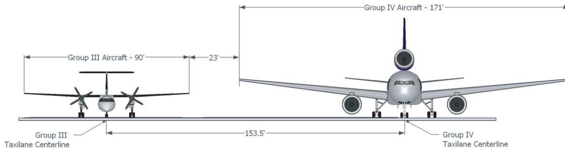
Figure H-1. Cross-section of existing separation at PHL.
