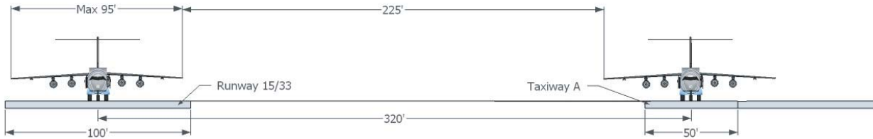
Figure H-16. Cross-section of existing separation at ASE.
