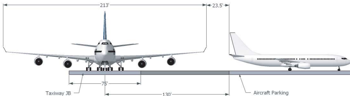
Figure H-8. Cross-section of existing separation at EWR.
