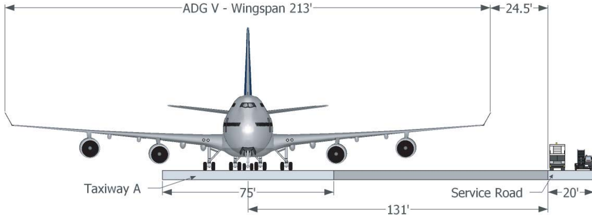
Figure H-10. Cross-section of the existing separation at ORD for Case Study # 10.
