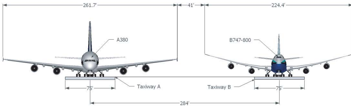
Figure H-7. Cross-section of existing separation at JFK.
