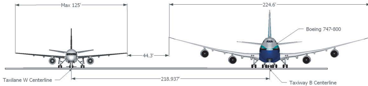
Figure H-15. Cross-section of the existing separation at SEA for Case Study # 15.
