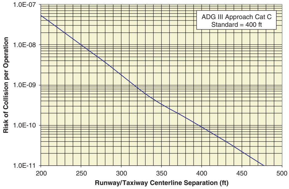
Figure AA-34. Missed approach collision risk for ADG III Cat II.
