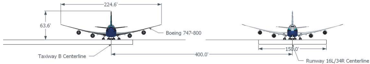
Figure H-14. Cross-section of the existing separation at SEA for Case Study # 14.
