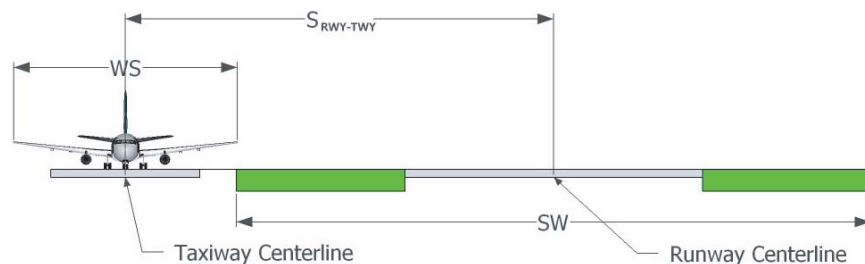
Figure 5. Runway/parallel taxiway separation distance.
