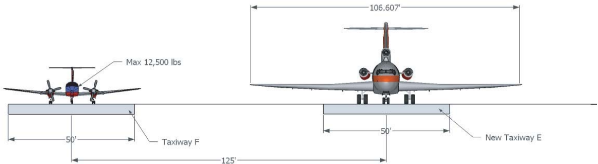
Figure H-17. Cross-section of the existing parallel taxiway separation at ACK.
