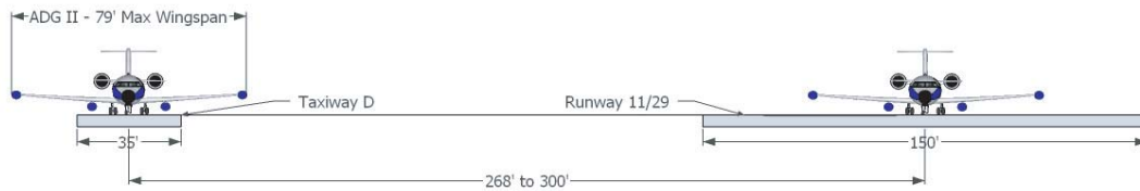
Figure H-4. Cross-section of existing separation at BDR.
