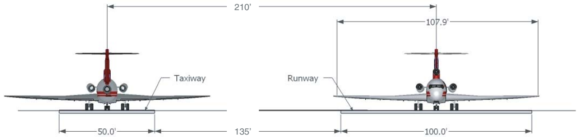
Figure H-13. Cross-section of the existing runway/taxiway separation at LCI.
