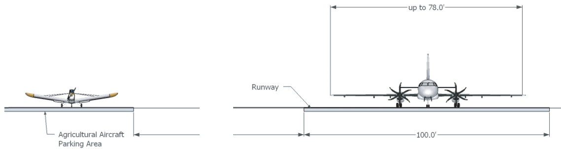
Figure H-5. Cross-section of existing separation at MFV.
