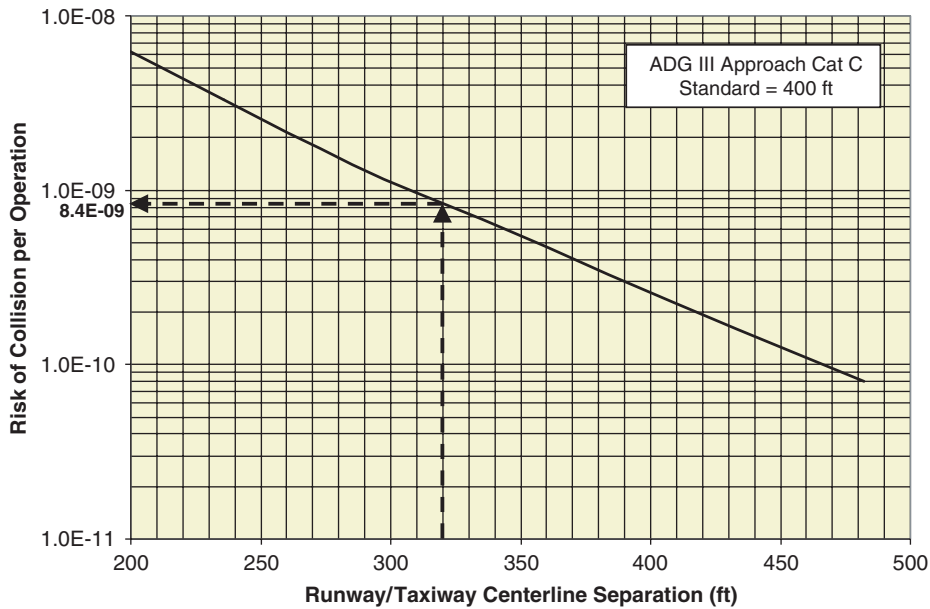
Figure A-14. Estimating airborne risk of runway/taxiway separation (ADG III-CAT I).
