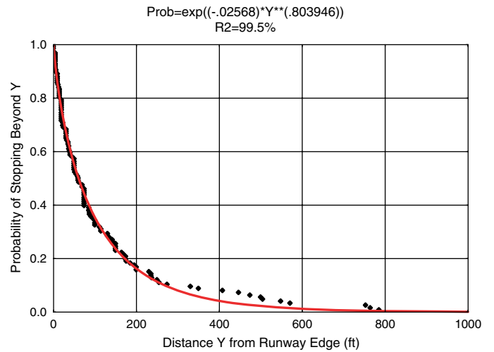
Figure 21. Location model for landing veer-off.
