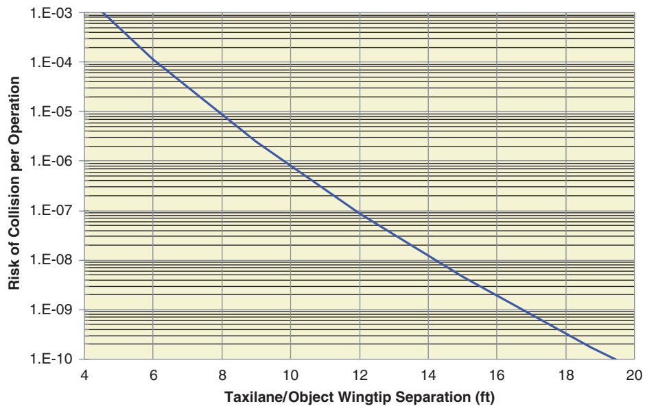
Figure 15. Taxilane/object collision risk based on wingtip separation.
