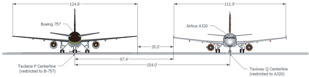
Figure H-9. Cross-section of the existing separation at MSP.
