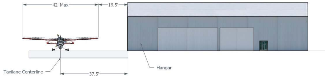
Figure H-6. Cross-section of existing separation at N07.
