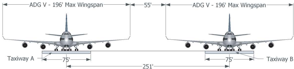
Figure H-11. Cross-section of the existing separation at ORD for Case Study # 11.
