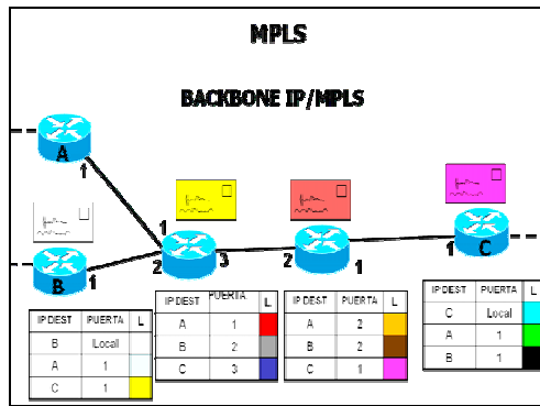
Figure 4-2: MPLS Switching
