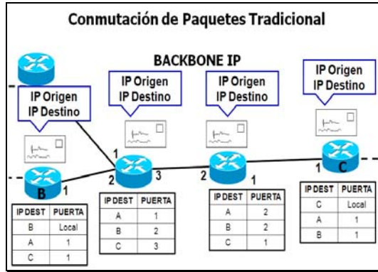
Figure 4-1: IP Switching
