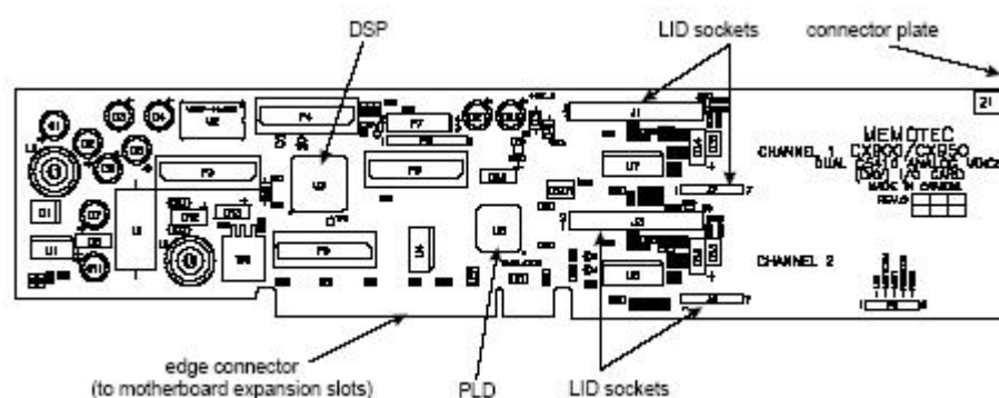
DAV I/O Card (without SLIM LIDs)
