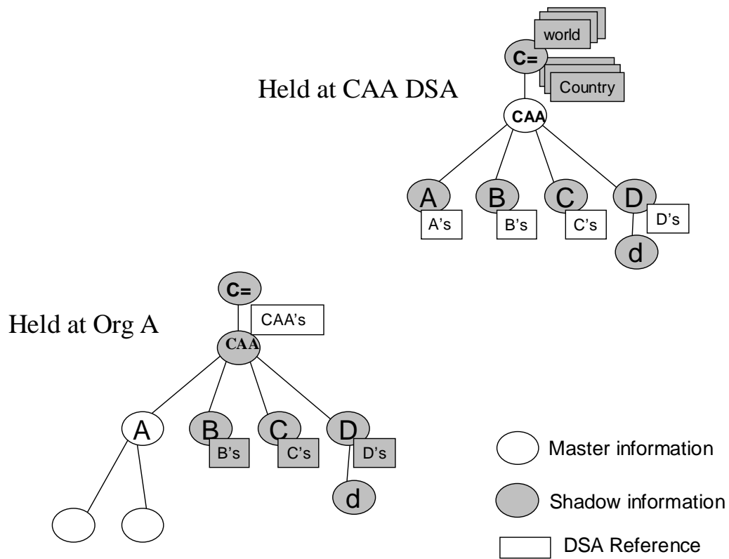
Figure 5.2-4: Minimum Information Mastered and Shadowed
