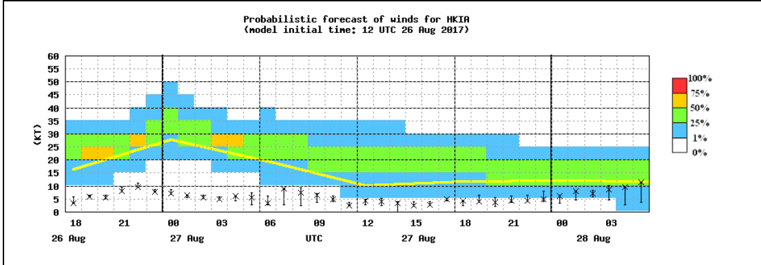
Figure 4. An example of probabilistic forecast of winds at HKIA during TC situation. The probability of wind speed with time are shown in colour. The deterministic model forecast (in yellow line) is also displayed on the time series plot for users' reference.
