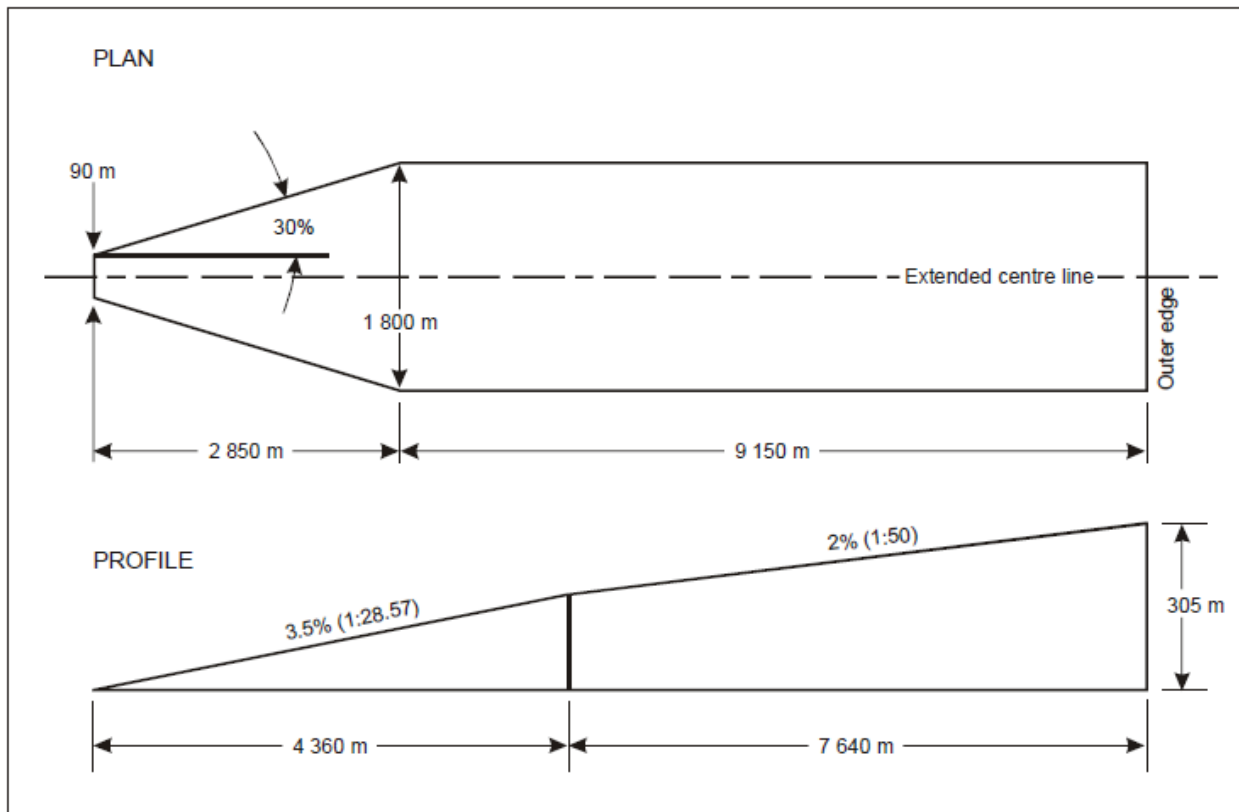
Figure A4-1. Take-off climb Surface for Instrument FATO
