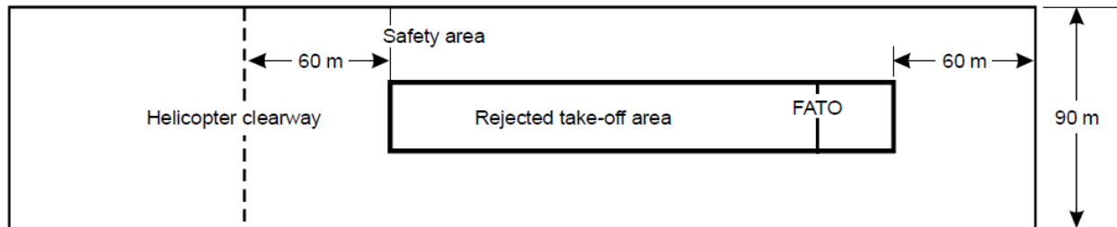
Figure A3-1. Safety Area for Instrument FATO
