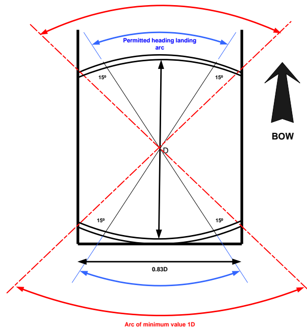
Figure 3-810. Shipboard permitted landing headings for limited heading operations
