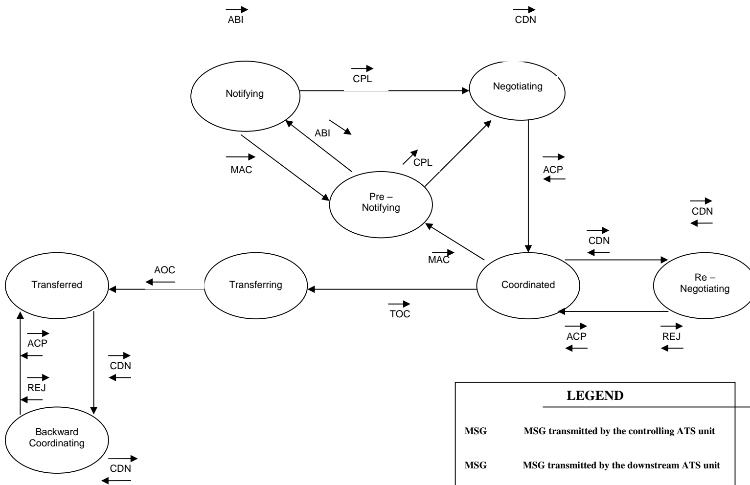
Figure D-2 Flight State Transition Diagram
