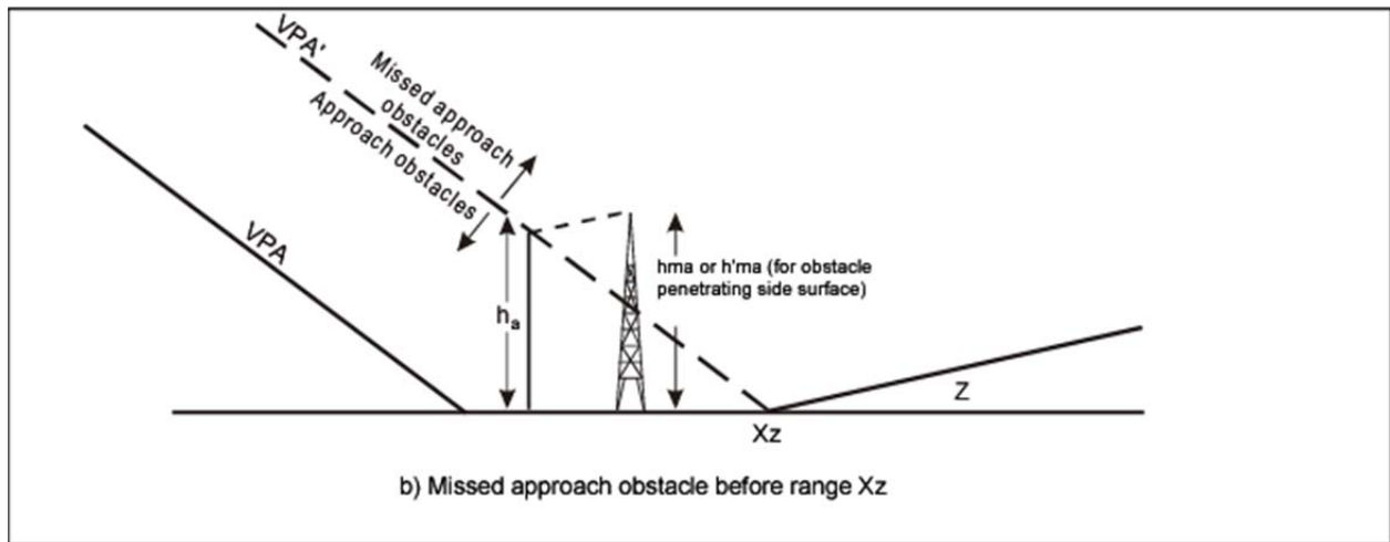
Figure III-3-4-5 a) and b). Missed approach obstacles
