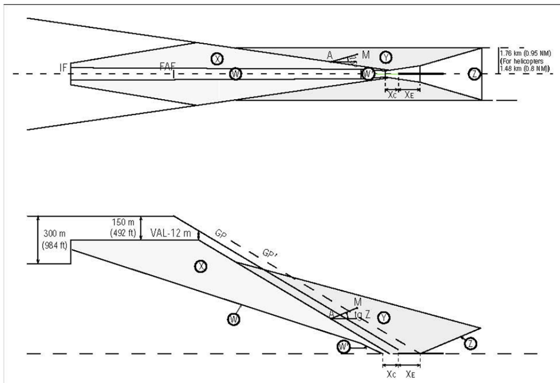
Figure III-Att-1. Illustration of SBAS APV obstacle assessment surfaces
