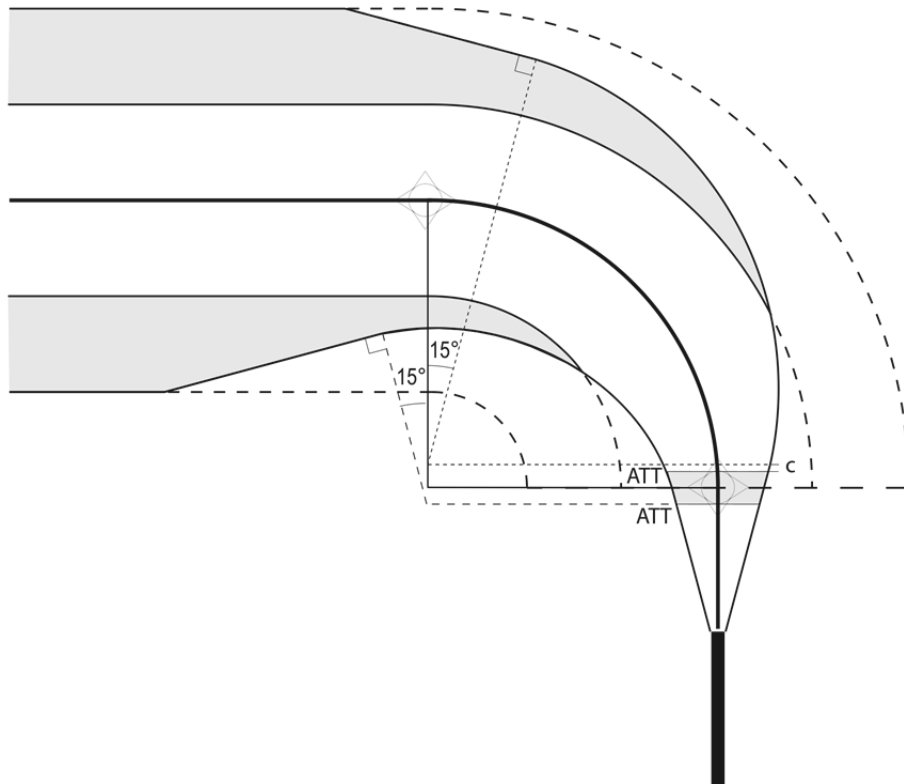
Figure III-2-2-14. Splay in RF turn
