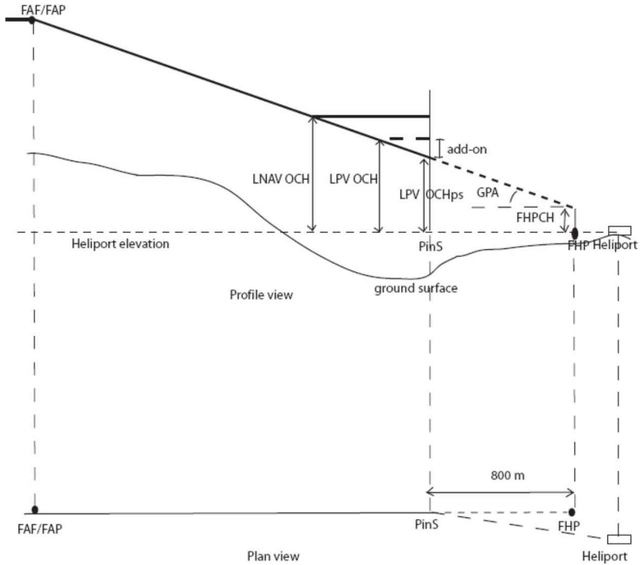
Figure IV-3-1. Representation of a PinS RNP APCH supporting LNAV and LPV minima
