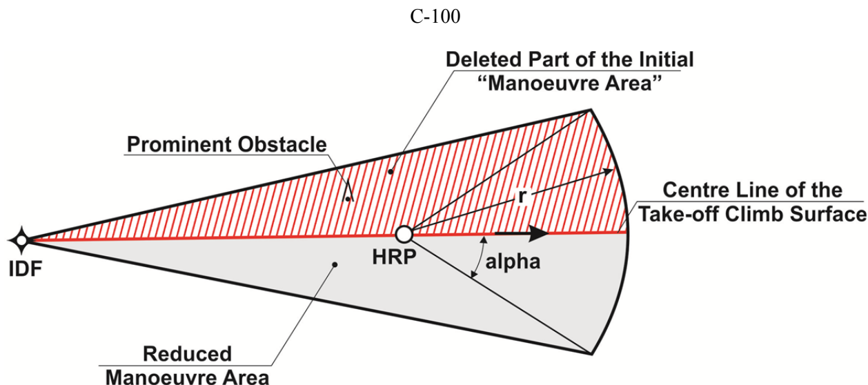
Reduction of the Manoeuvring area due to a prominent obstacle (left turn prohibited)
