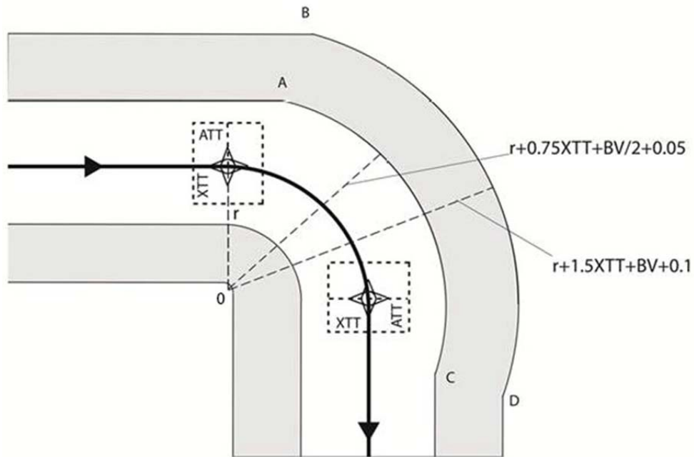
Figure III-2-2-13. RF turn protection
