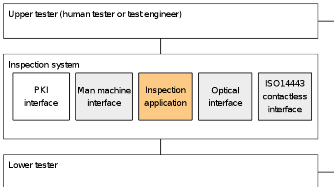
Figure 1: Upper and lower tester of the test environment
