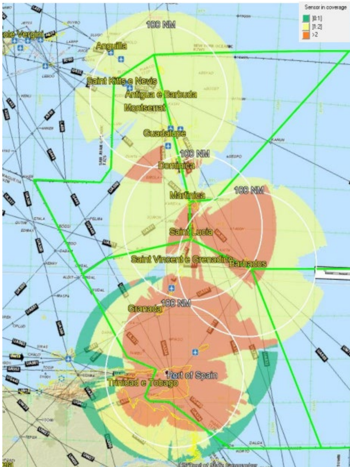
ADS-B coverage @4000 feet ASL
