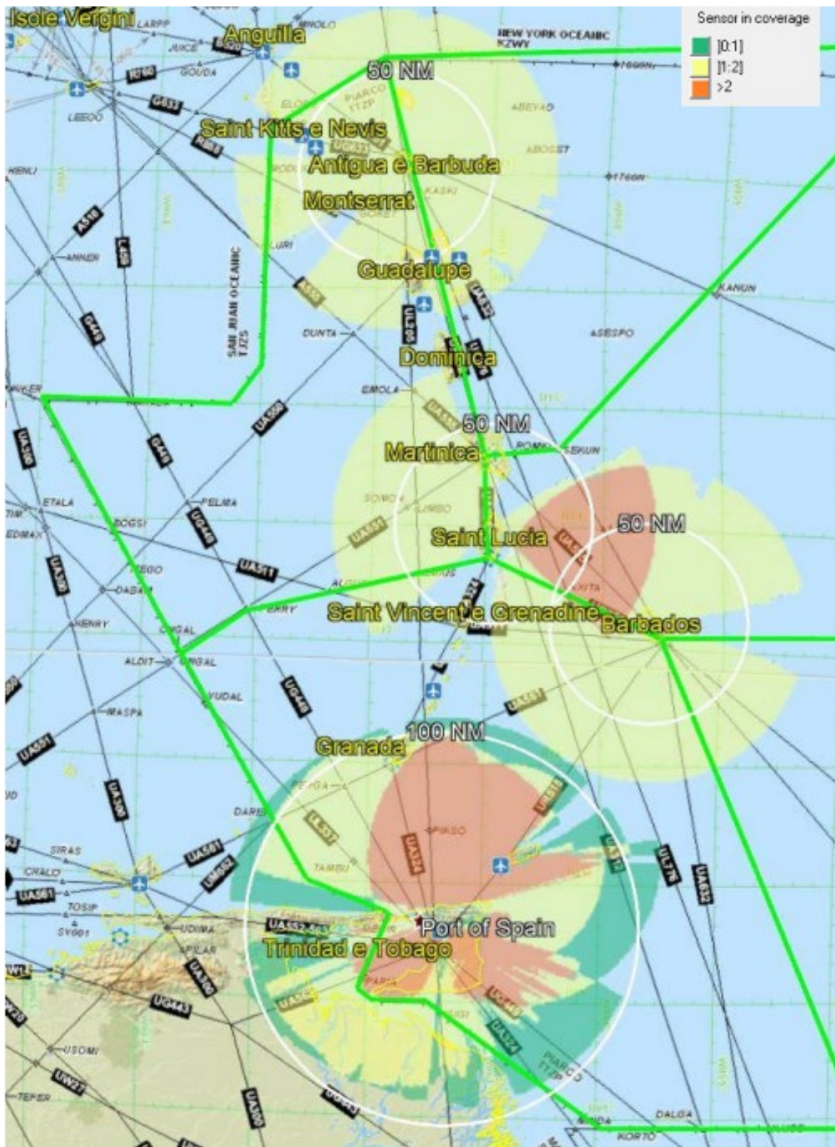
ADS-B coverage @1000 feet ASL
