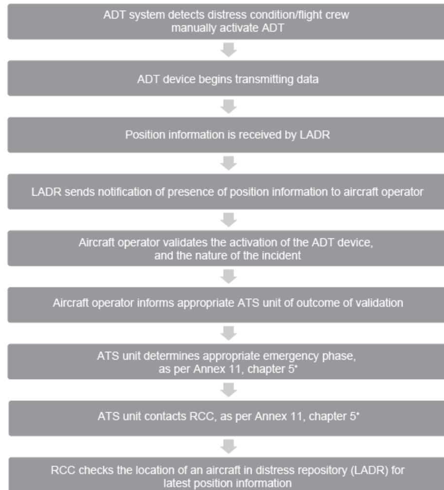
Figure V-1 – Schematic sequence of events arising from an autonomous distress tracking device activation
