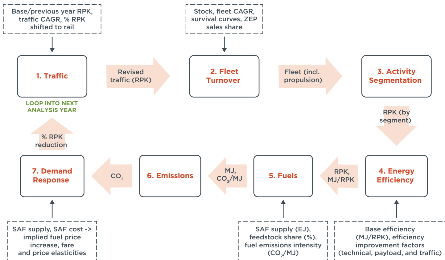
Figure 1. PACE model
