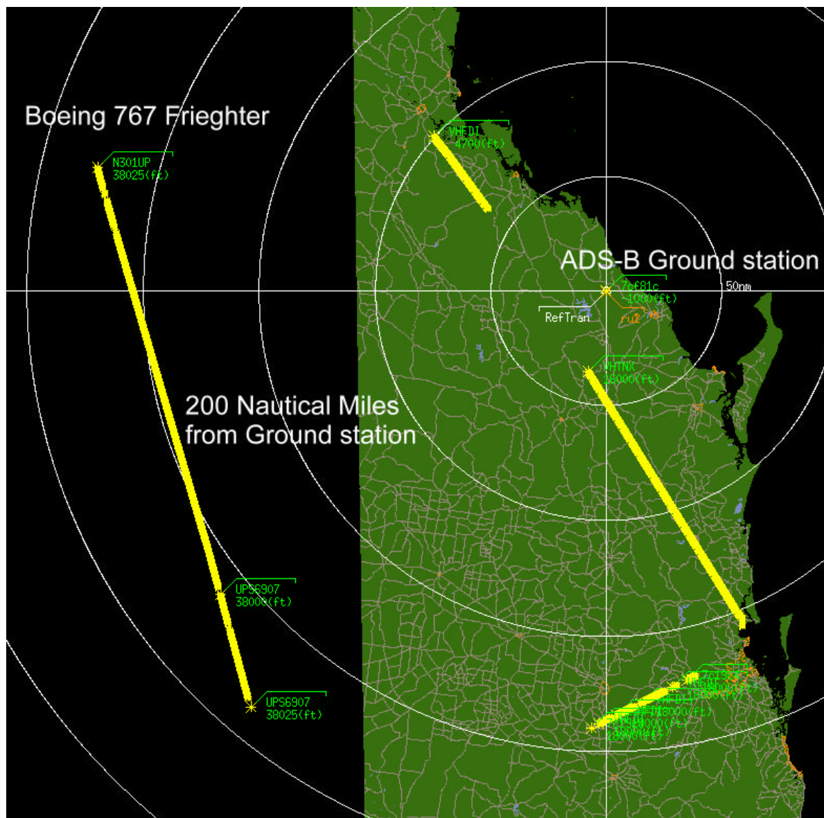
Figure 2. Illustrating coverage obtained from a single ground station. At FL 380 this Boeing 767 ADS-B equipped aircraft was tracked beyond 220 NM. The Boeing 767 is operated by UPS and is not part of the Australian ADS-B trial. UPS is presently equipping more than 100 aircraft with ADS-B.
