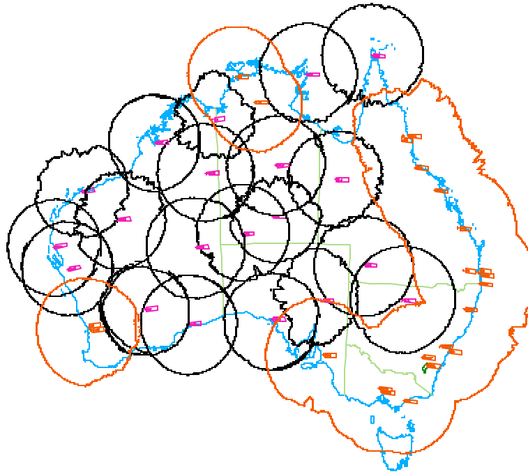
Figure 3. Proposed composite radar and ADS-B coverage at FL 300 after deployment of 20 ADS-B sites.
