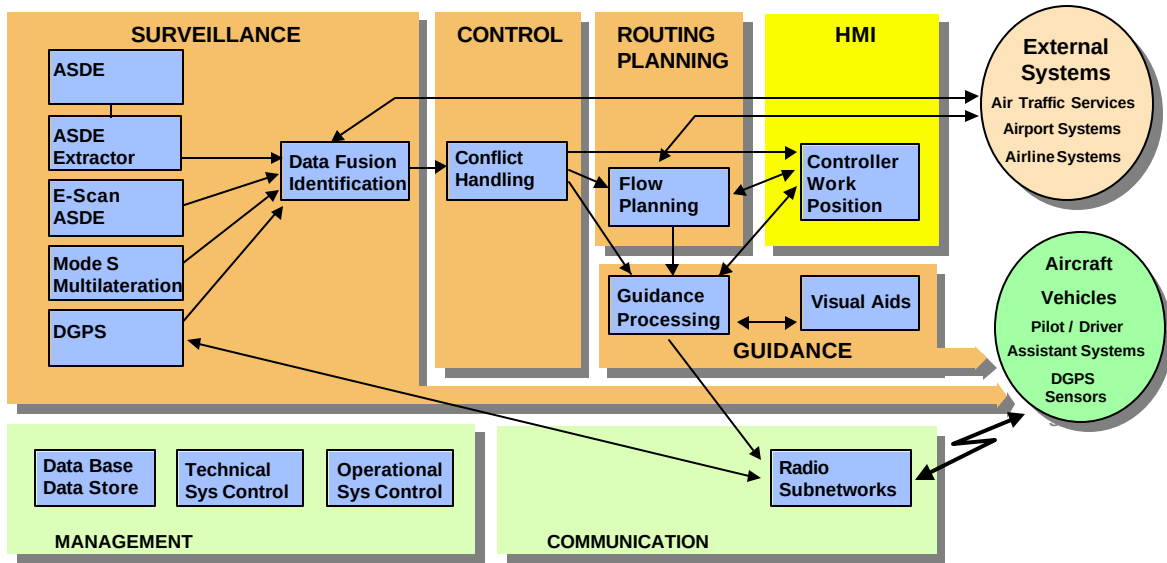
Figure 4. DEFAMM functional architecture
