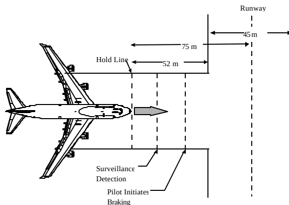
Figure 3-1. Runway incursion detection scenario
