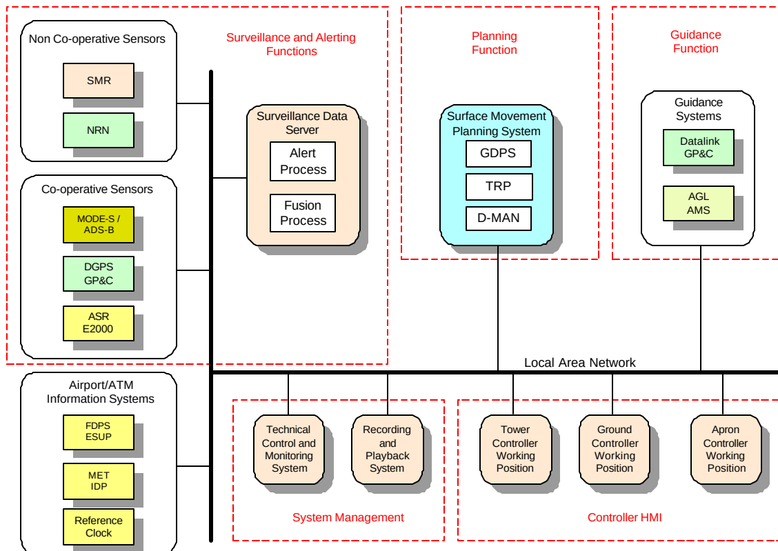
Figure 5. BETA functional architecture
