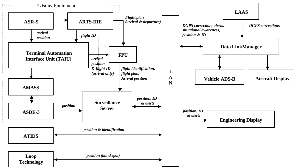
Figure 6. RIRP system block diagram
