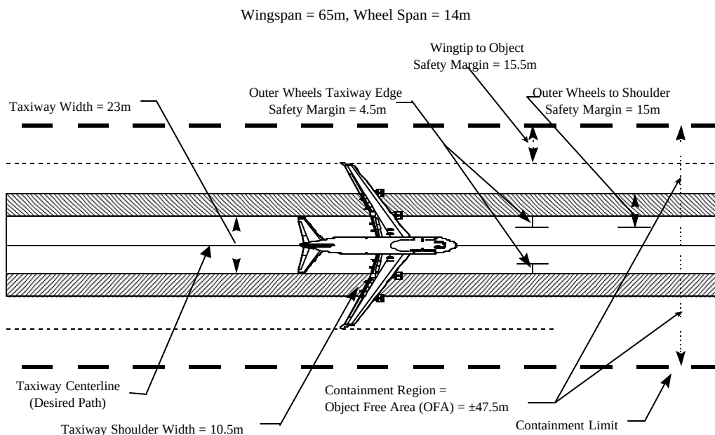
Figure 7. Taxiway design standards for aerodrome Code letter E aircraft
