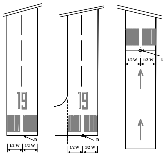
Figure 3-4. Topography points - thresholds
