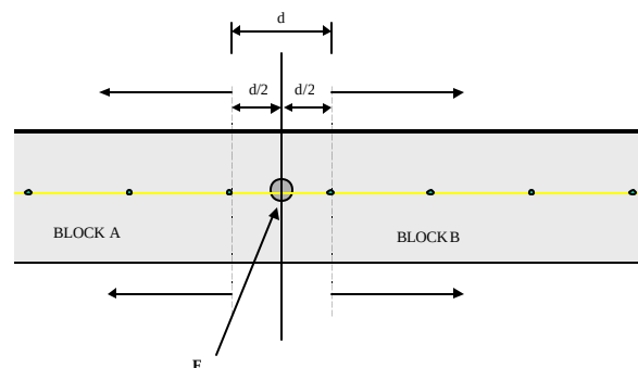
Figure 3-7. Topography points - taxiway blocks
