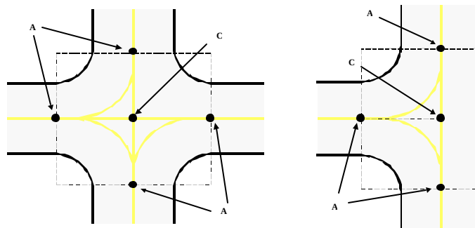
Figure 3-6. Topography points - taxiway intersections
