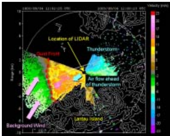
Figure 3 – LIDAR Doppler velocity display at 1.0 degree elevation, revealing a gust front (red dotted line) with about 35 knots wind speed gain across.
