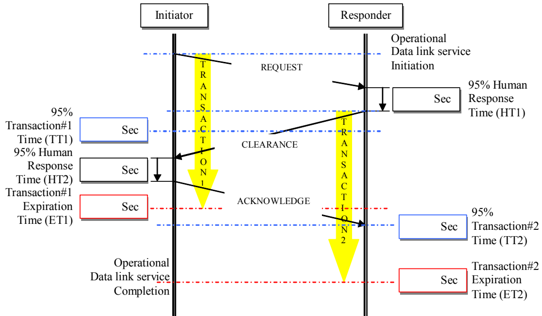
Fig.3-9 Time related Operational Performance Parameters © 2000 RTCA, Inc
