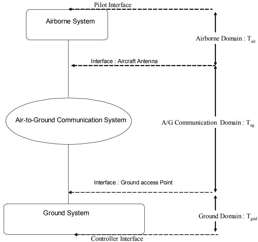
Fig.3-5 Technical Performance and Allocation to Domains
