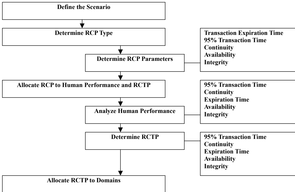
Fig.4-1 Suggested (Detailed) Process of Operational Performance Determination
