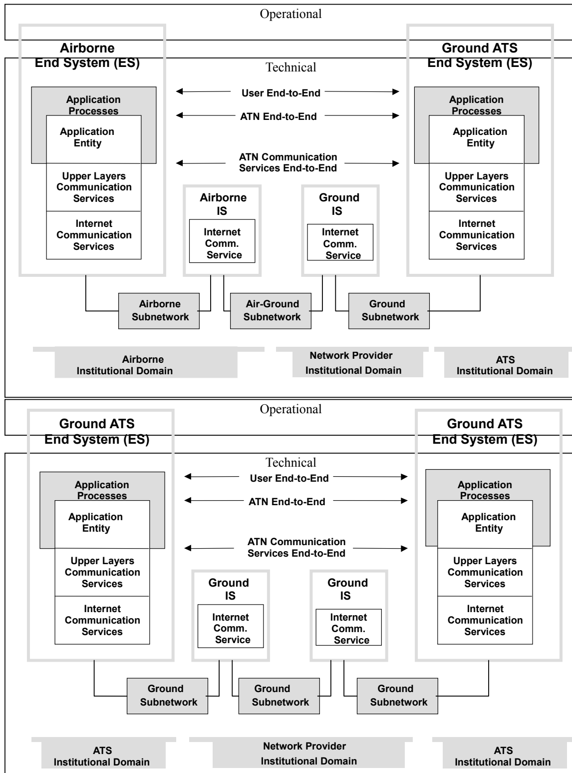
Fig.3-7 Technical Components of Air-Ground and Ground-Ground Communication
