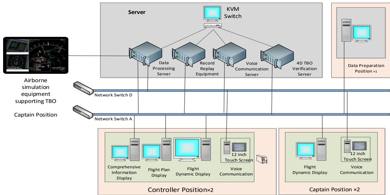
Figure 1. Structure diagram of TBO simulation and validation platform
