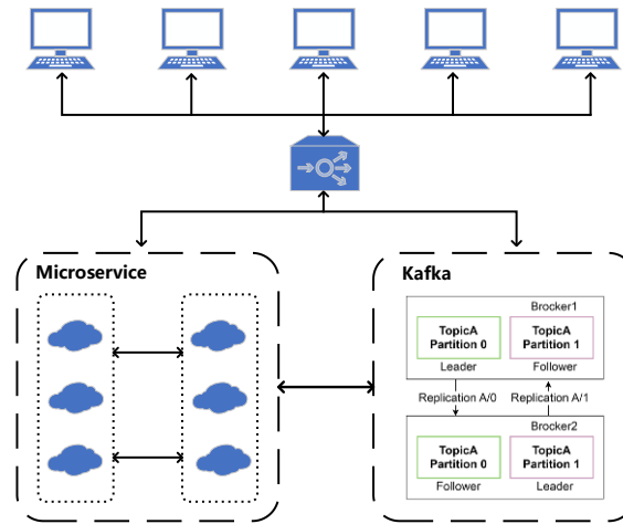
Figure 3 New SWIM Architecture
