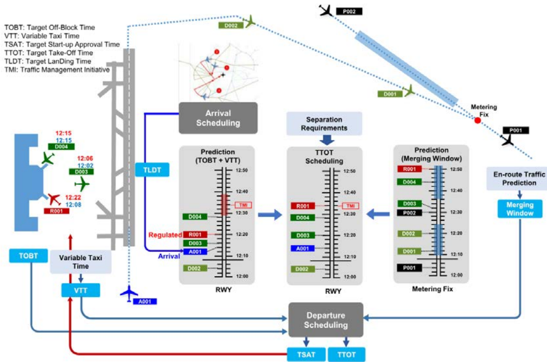
Figure 2. Operational Concept of MIDAS
