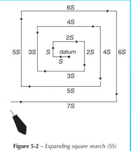
Figure 5-2 – Expanding square search (SS)
