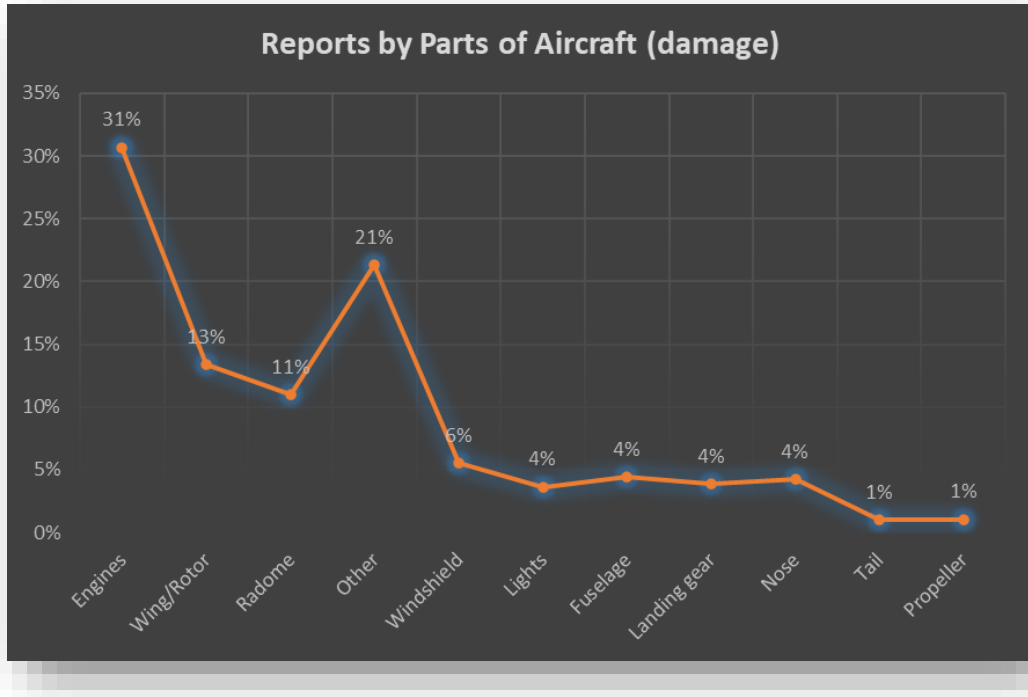
Chart E-18. Wildlife strikes reported by parts of aircraft (damage) in the EUR/NAT region
