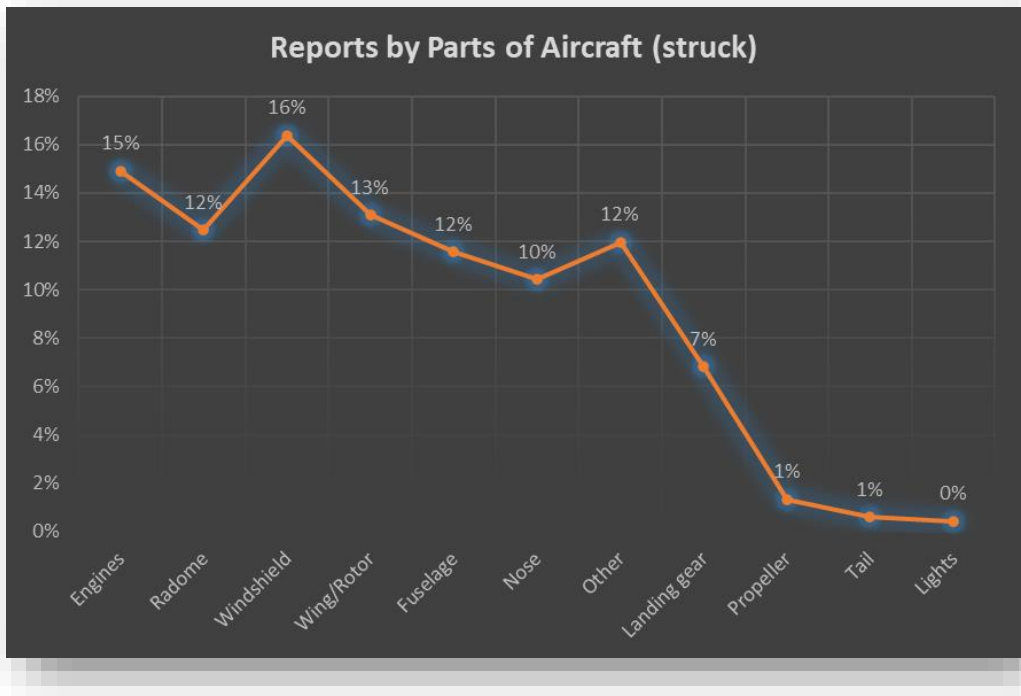
Chart E-17. Wildlife strikes reported by parts of aircraft (struck) in the EUR/NAT region
