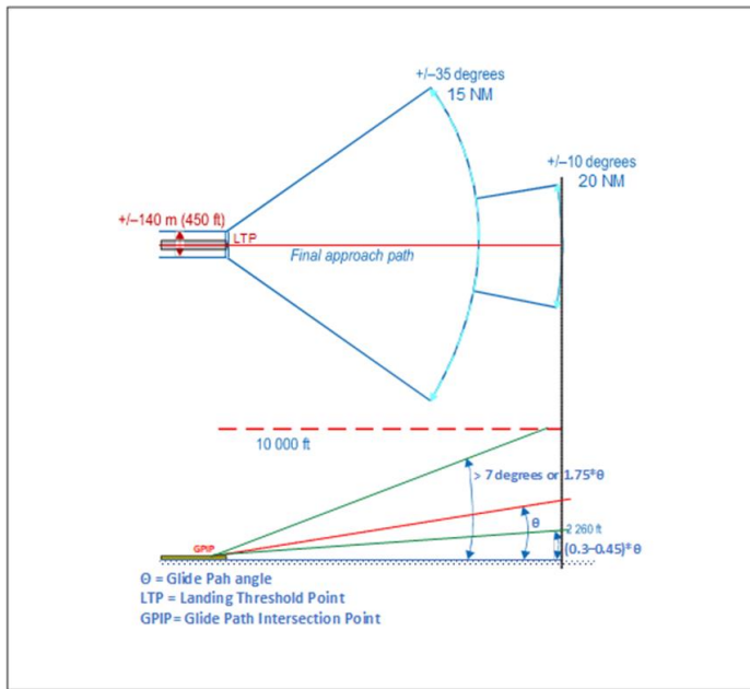
Figure 4-333 Minimum required DOC of GBAS
