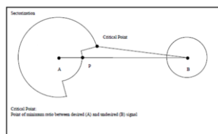
Figure 4-2 Geometry for determining the test points
