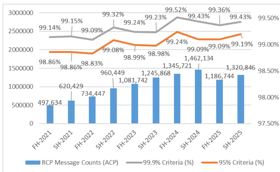
Figure 3: Number of RCP Message Counts, and Percentage Meeting 95% and 99.90% Criteria (ACP)
