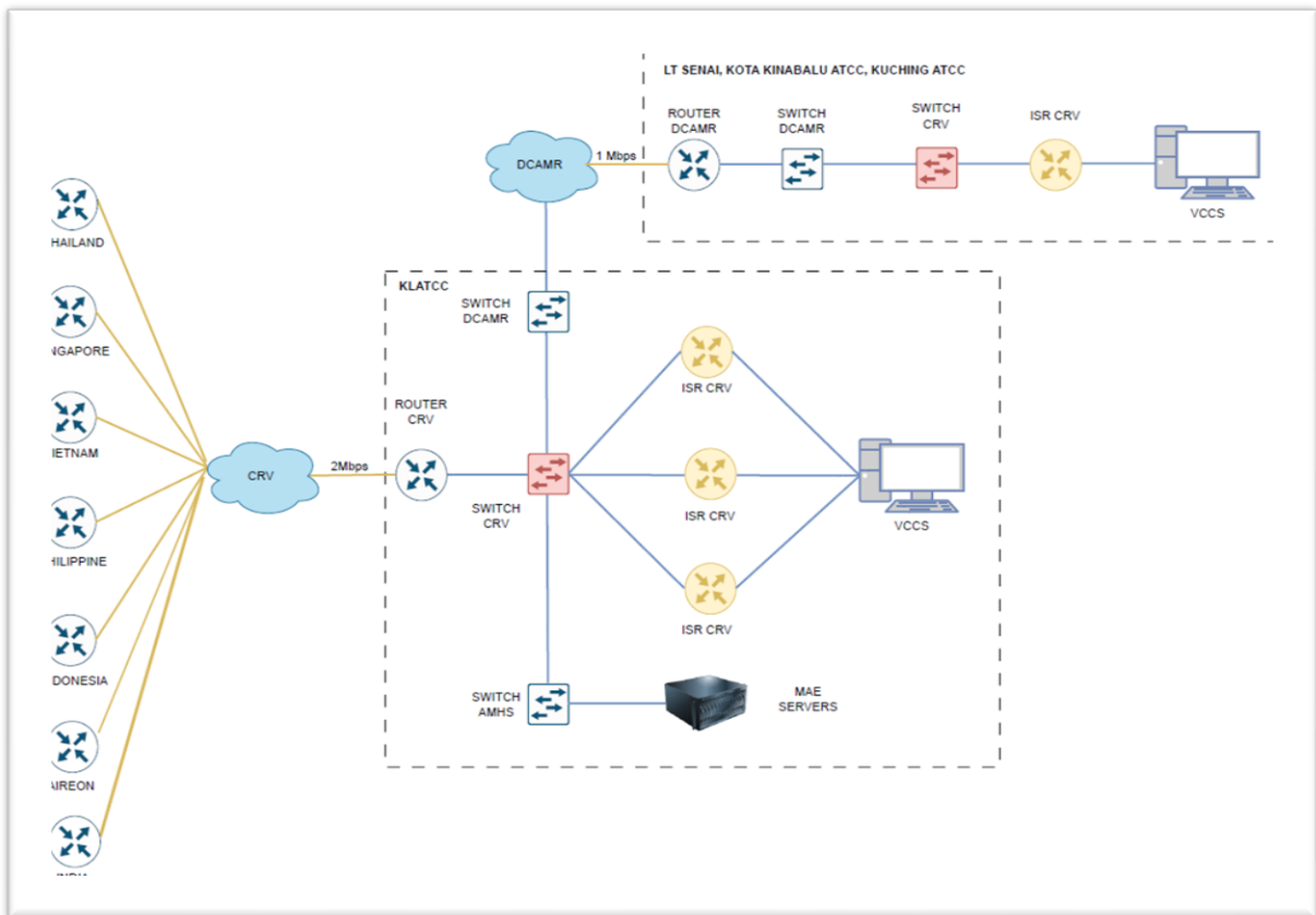
CRV Network Diagram – Kuala Lumpur Air Traffic Control Centre (KLATCC)
