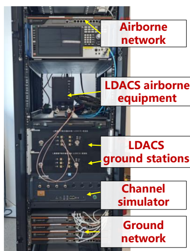
Figure 1 LDACS airborne and ground systems
