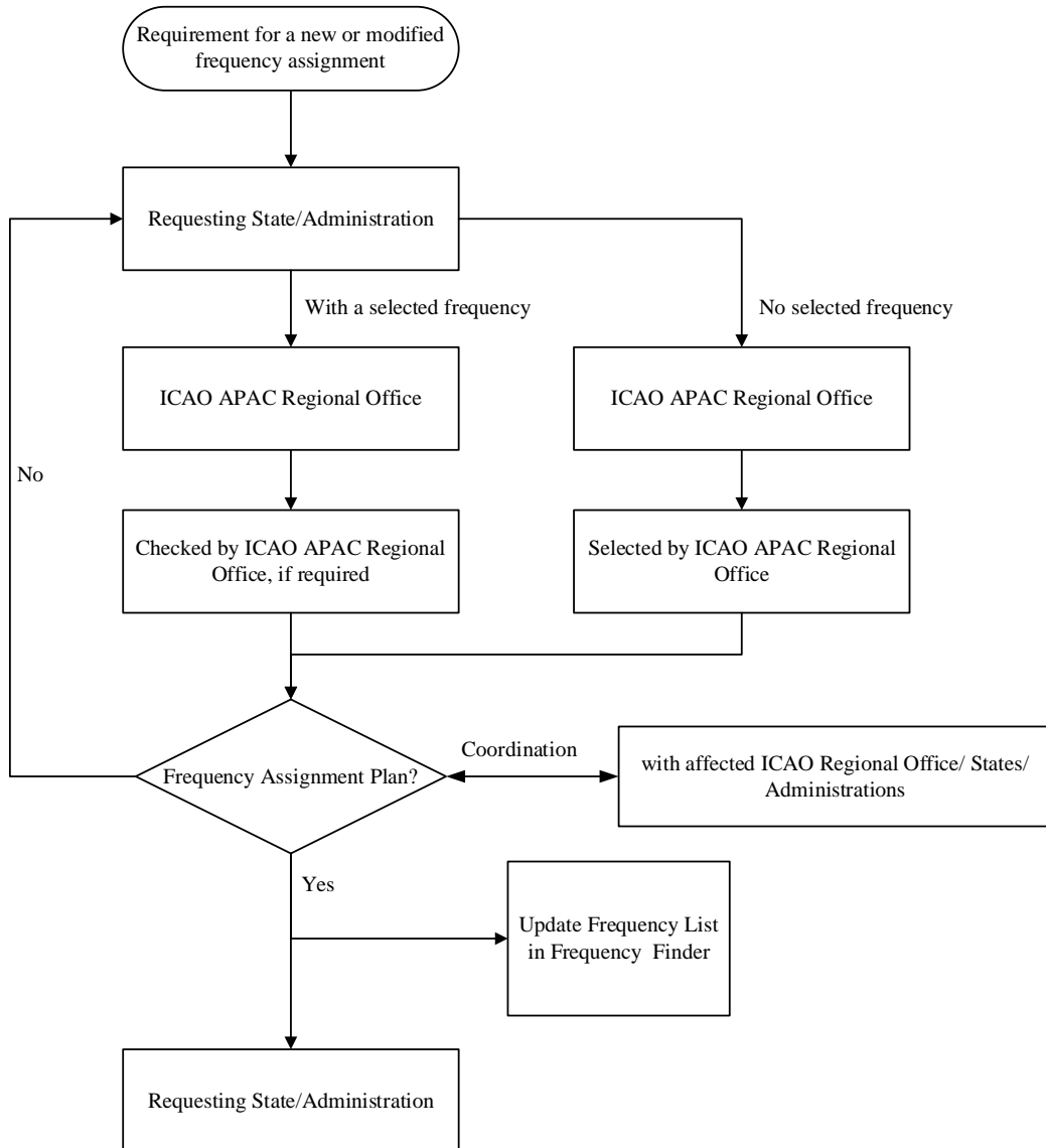
Figure 2-1 The basic aeronautical coordination procedure
