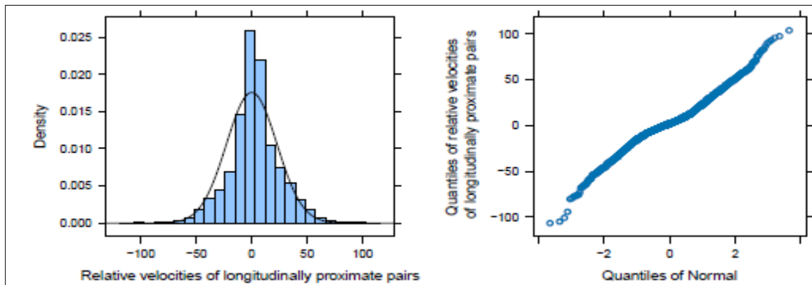
Figure 6: Distribution of relative velocities of longitudinally proximate pairs. The Normal distribution does not necessarily seem to be a reasonable fit.
