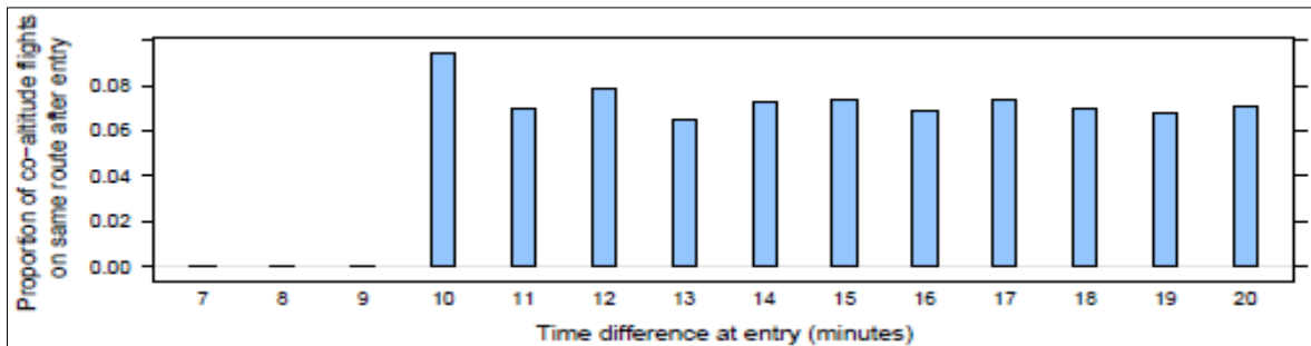
Figure 5: Values of Q(k) estimated from TSD. For co-altitude flights on the same route (after entry / before exit), the proportion of flights that entered k minutes after the preceding flight is plotted for k = 7,8,9,.....20 minutes.
