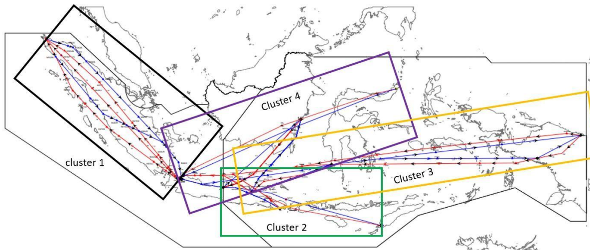
Figure 2. Design of PBN Domestic Enroute RNAV 2
