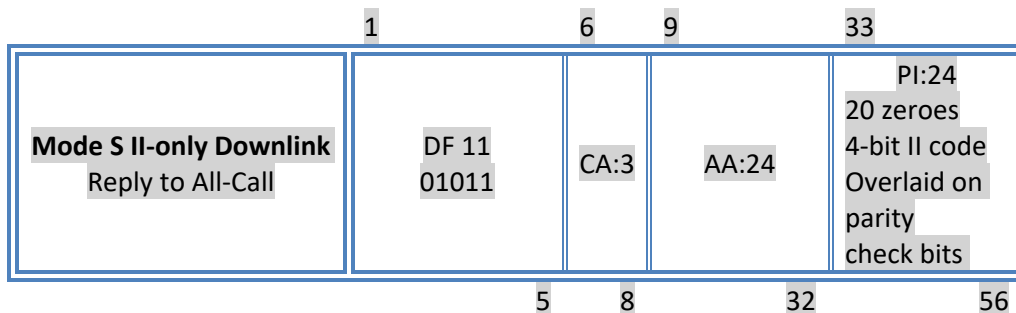
Figure J-18/1 All-Call reply from Mode S II-only transponder, downlink format 11
