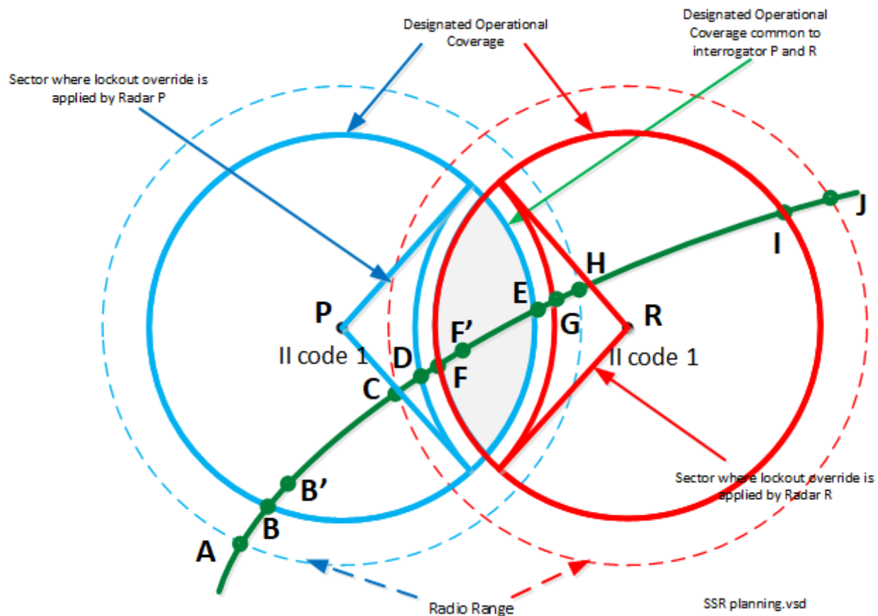
Figure J-23. Lockout override
