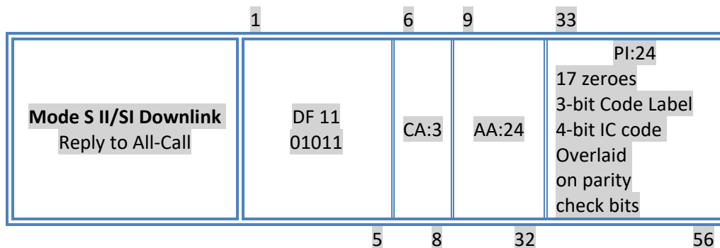
Figure J-18/2 All-Call reply from Mode S II/SI transponder, downlink format 11
