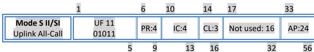
Figure J-17/2 Mode S All-Call structure for Mode S II/SI all-call (Uplink format 11 current definition)
