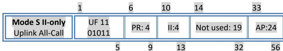
Figure J-17/1 Mode S All-Call structure for Mode S II-only all-call (Uplink format 11 old definition)
