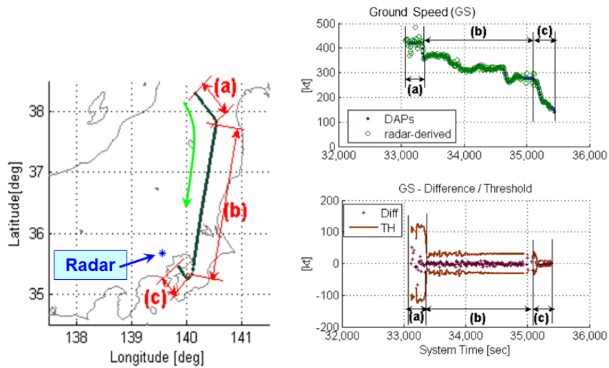
Figure 2 - Example of Dynamic Value Tests
