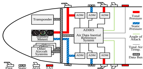
Figure 3.10 Typical ADIRS Architecture
