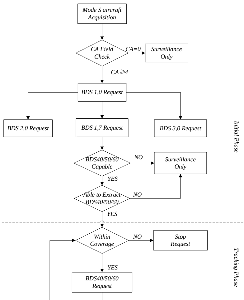
Figure.7-2 The Typical Procedure of DAPs Extraction
