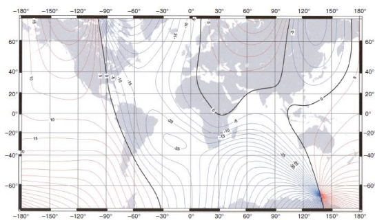
Figure 3.9 World Magnetic Model 2000
