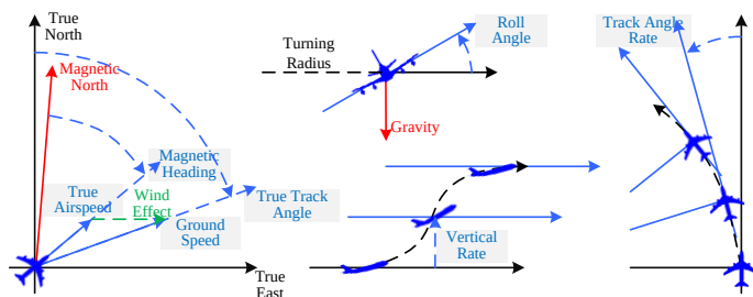
Figure 3.11 Illustration of Aircraft Dynamic
