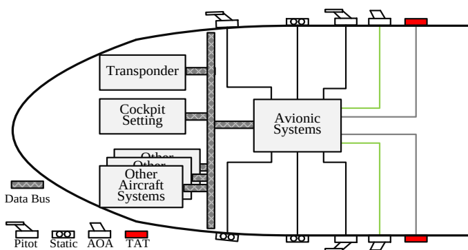
Figure 3.1 Typical DAPs Data Source Block Diagram
