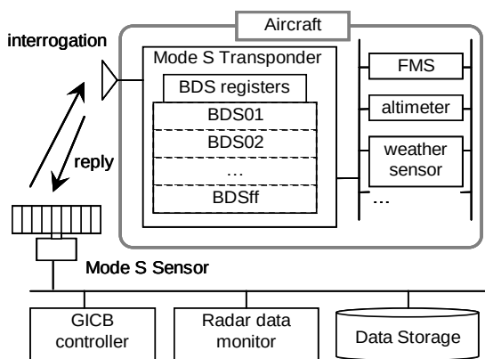
Figure1 - Example of Data Recording Configuration
