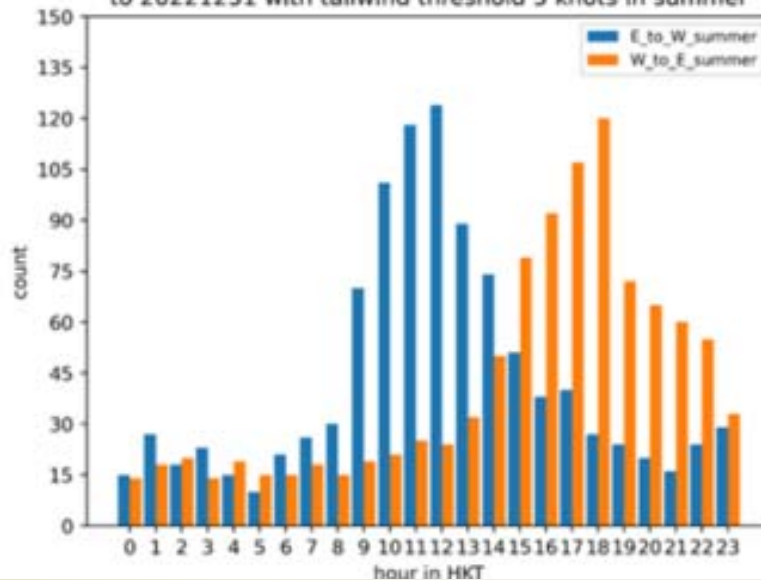
Hourly distribution of E_W_wind_change at r2w from 20160401 to 20221231 with tailwind threshold 5 knots in summer
