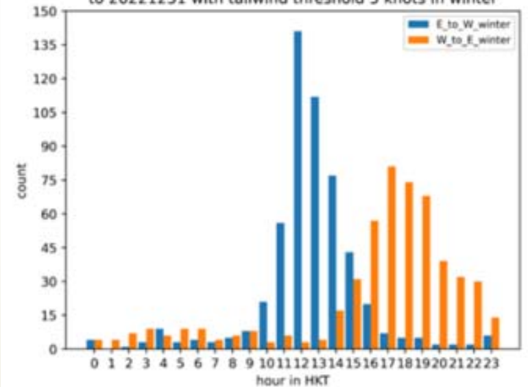
Hourly distribution of E_W_wind_change at r2e from 20160401 to 20221231 with tailwind threshold 5 knots in winter
